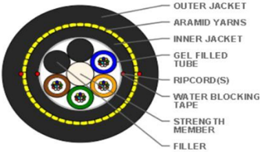
* Typical Construction Diagram - Not to Scale
